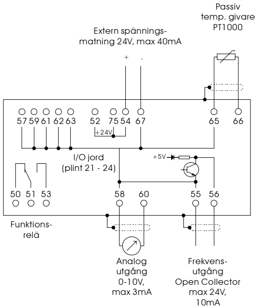
Figur 5. Inkoppling expansionskort
